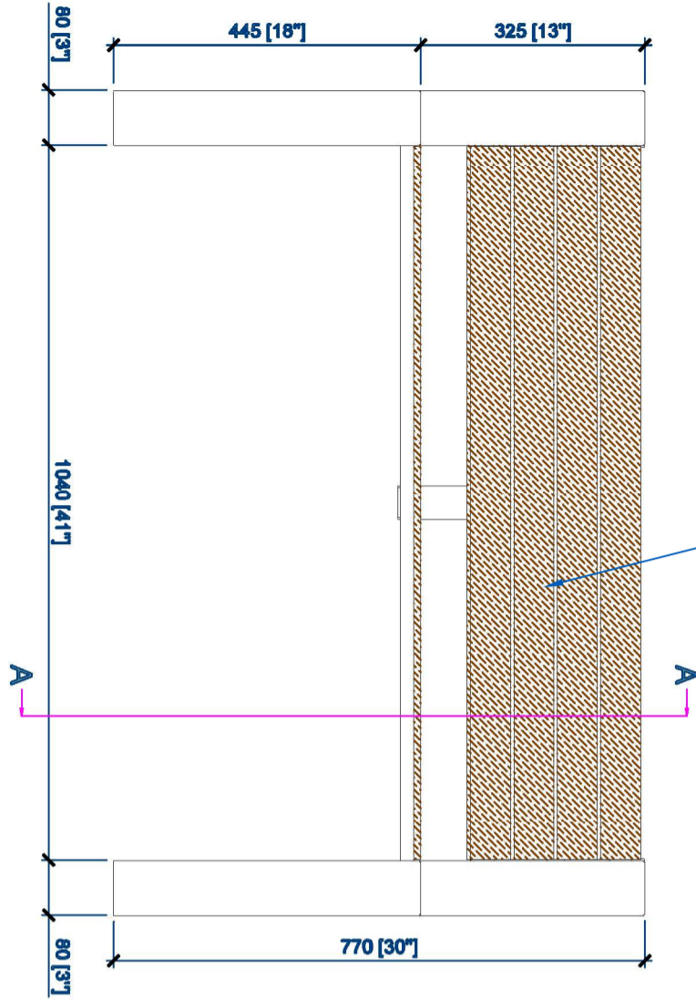
FRONTAL VIEW ALZADO FRONTAL
